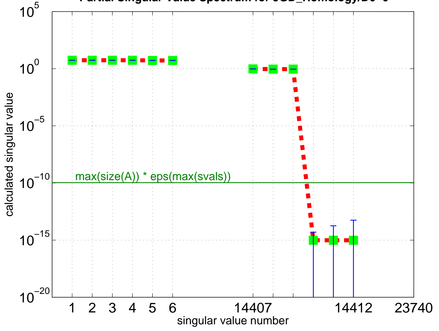
Partial Singular Value Spectrum for JGD_Homology/D6-6
