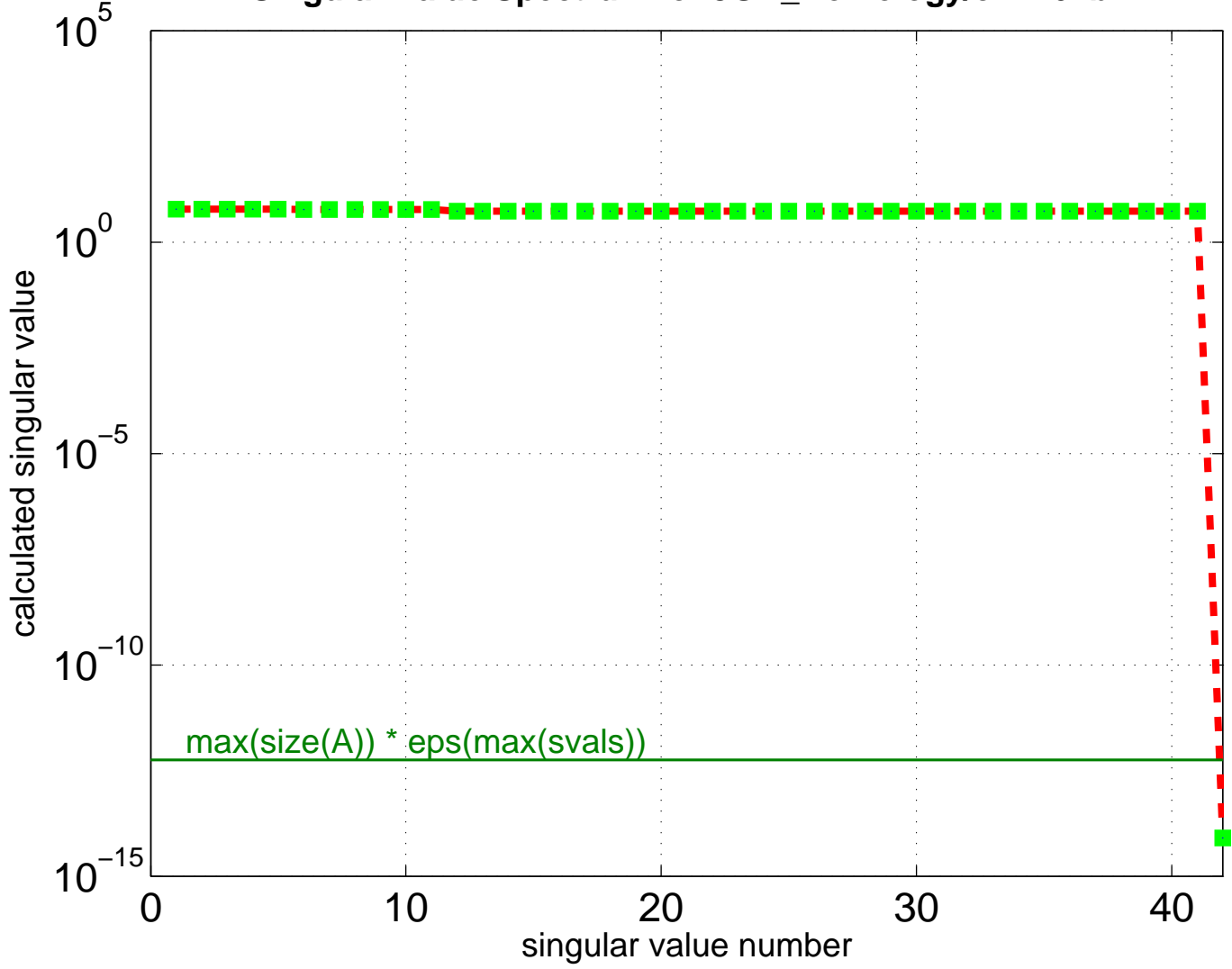
Singular Value Spectrum for JGD_Homology/ch7-6-b1
