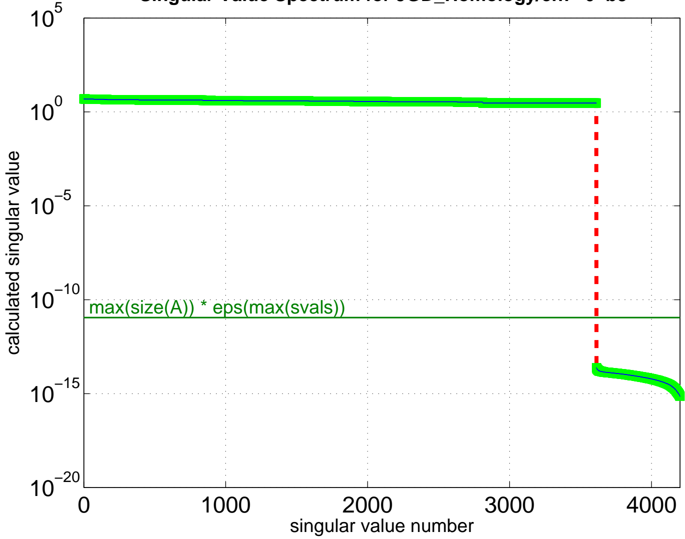
Singular Value Spectrum for JGD_Homology/ch7-6-b3
