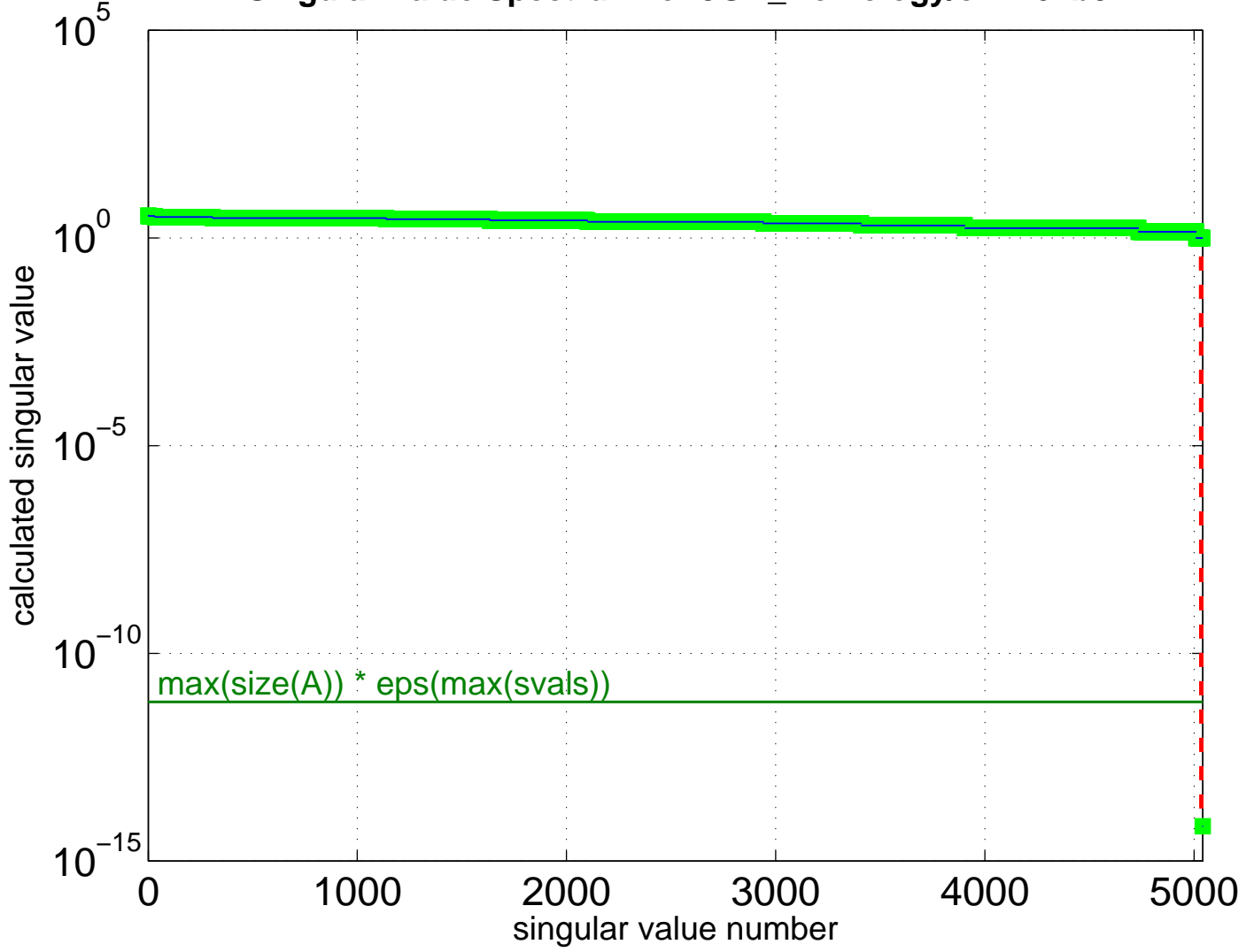
Singular Value Spectrum for JGD_Homology/ch7-6-b5
