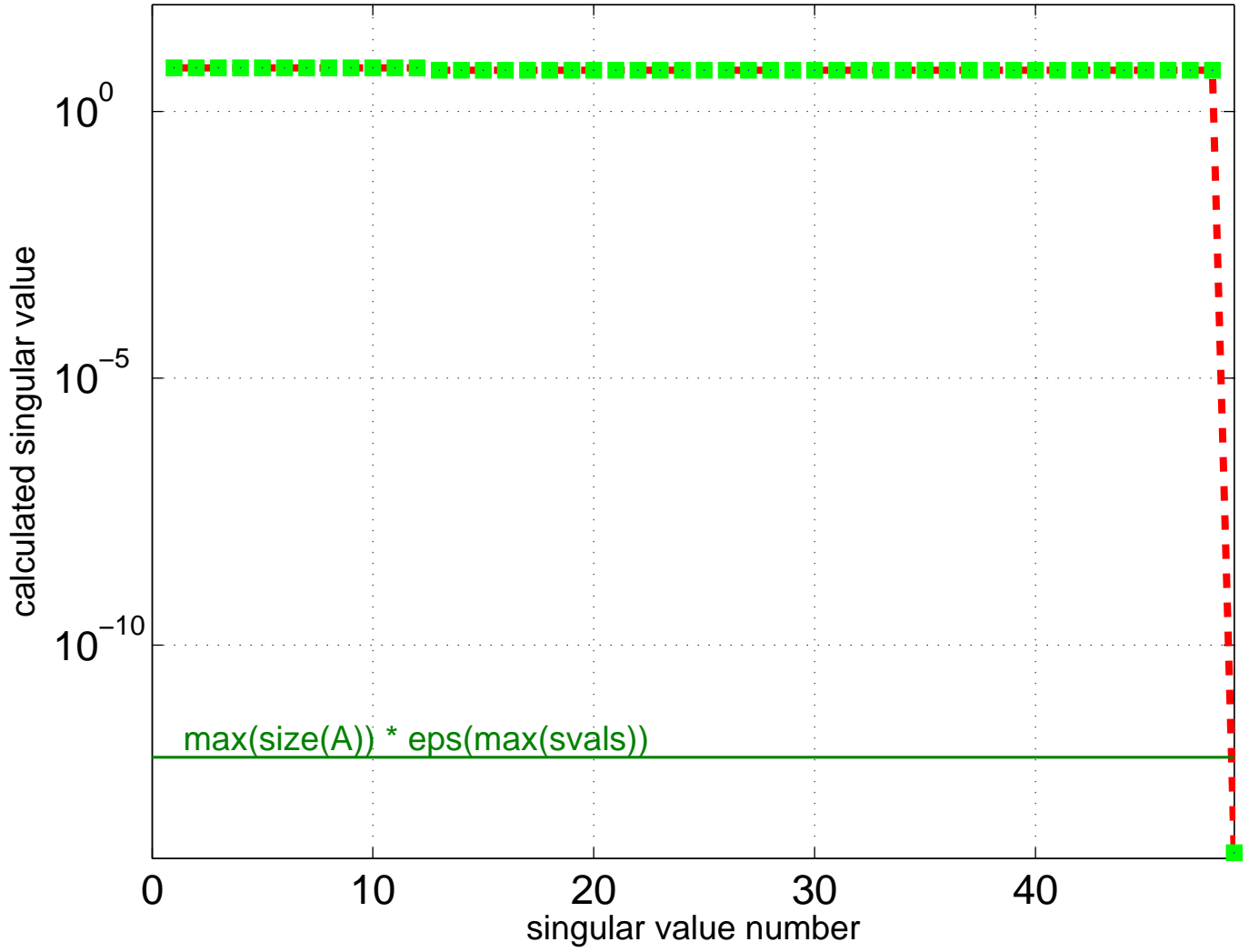
Singular Value Spectrum for JGD_Homology/ch7-7-b1
