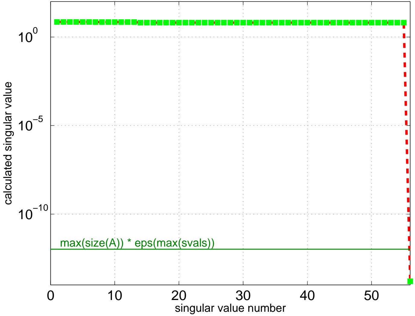
Singular Value Spectrum for JGD_Homology/ch7-8-b1
