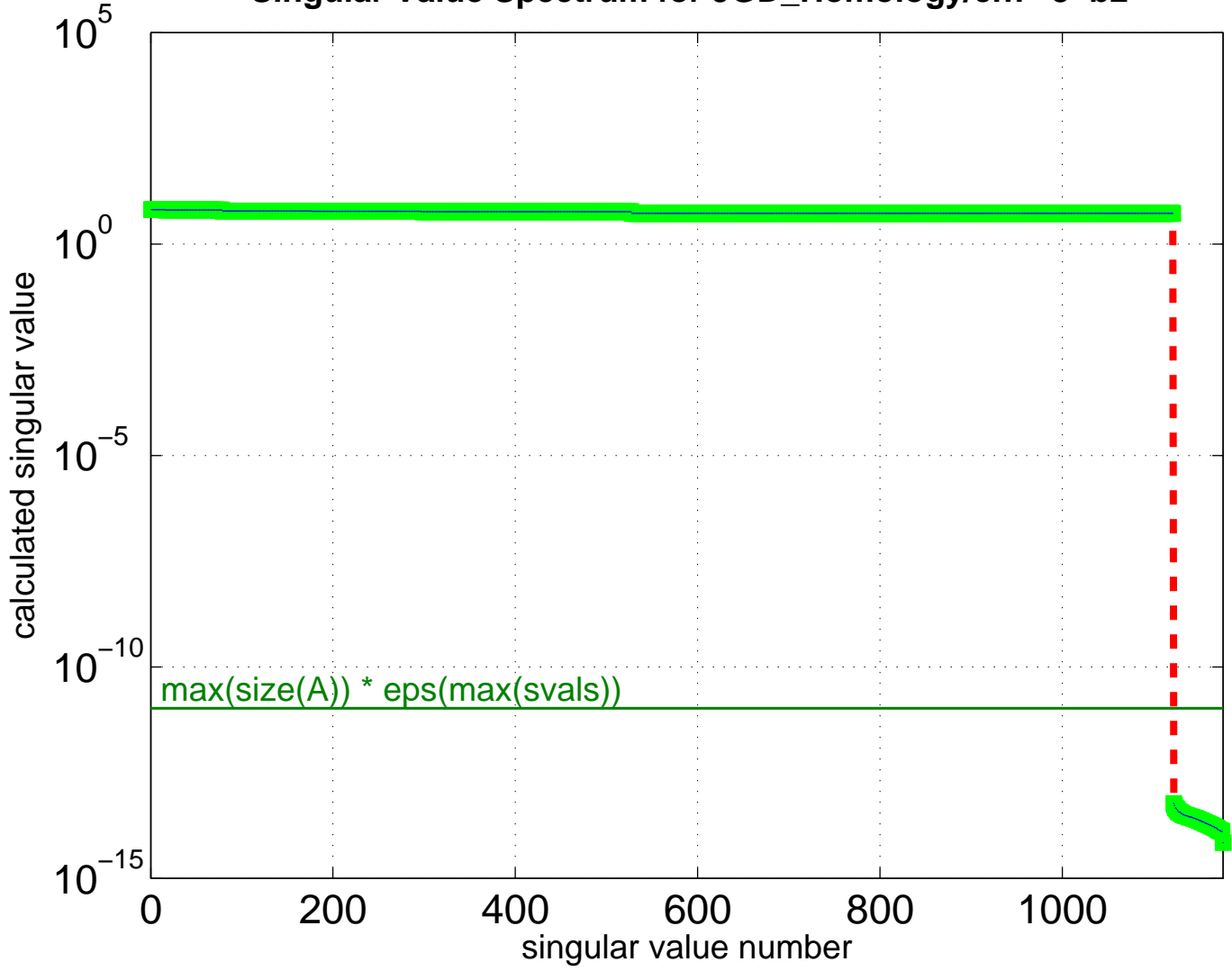
Singular Value Spectrum for JGD_Homology/ch7-8-b2
