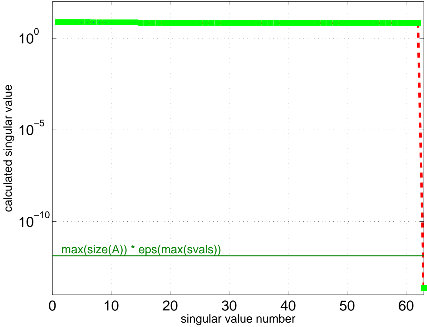
Singular Value Spectrum for JGD_Homology/ch7-9-b1
