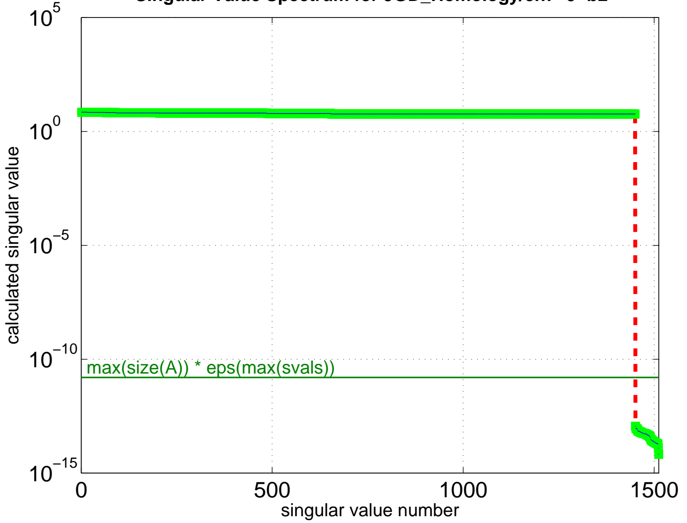
Singular Value Spectrum for JGD_Homology/ch7-9-b2
