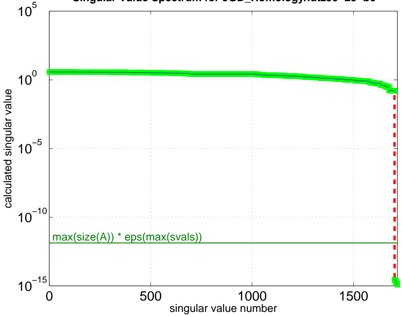
Singular Value Spectrum for JGD_Homology/lutz30-23-b6
