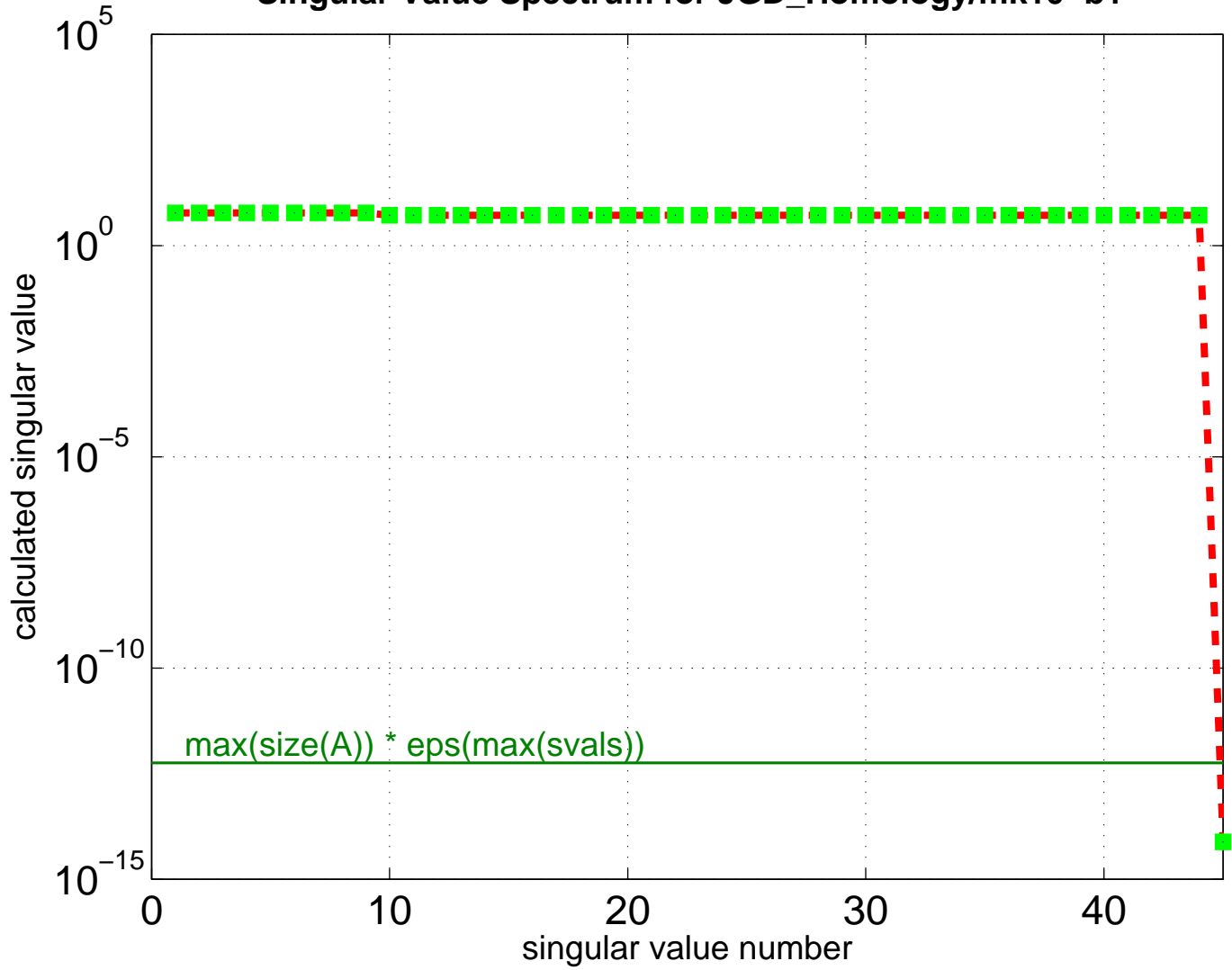
Singular Value Spectrum for JGD_Homology/mk10-b1
