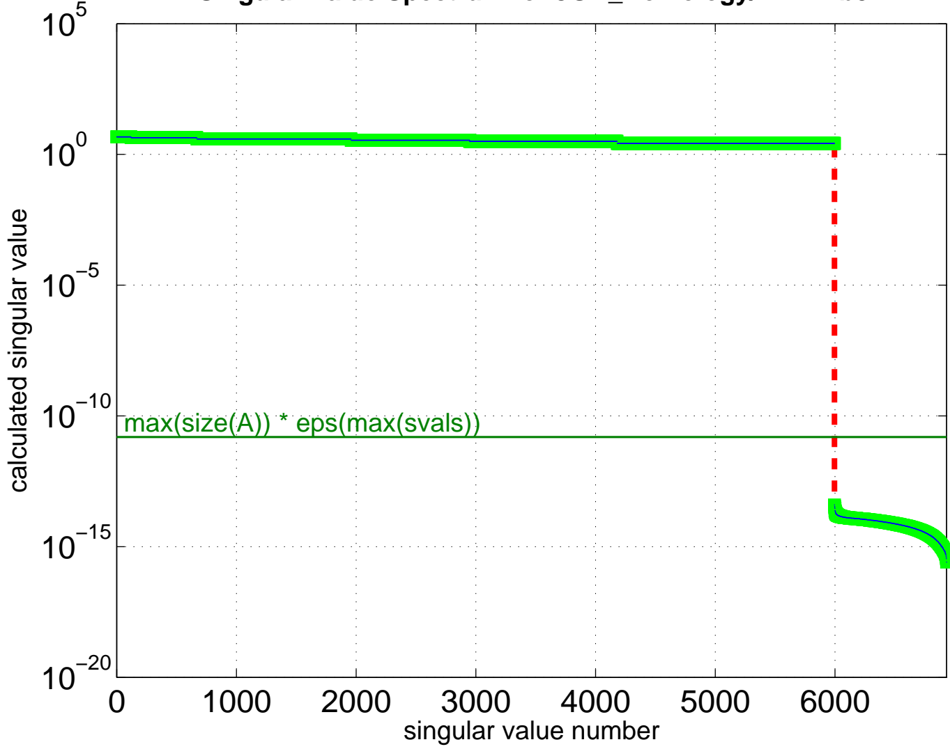
Singular Value Spectrum for JGD_Homology/mk11-b3
