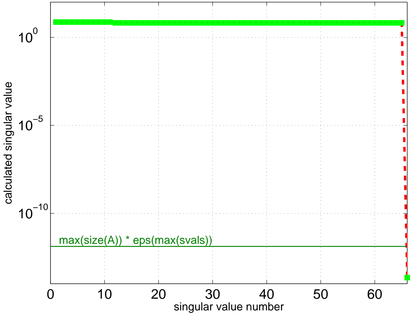
Singular Value Spectrum for JGD_Homology/mk12-b1
