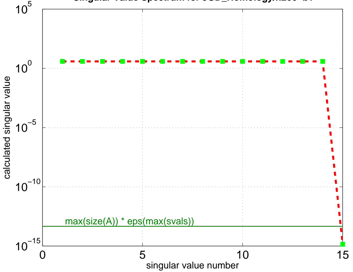
Singular Value Spectrum for JGD_Homology/n2c6-b1
