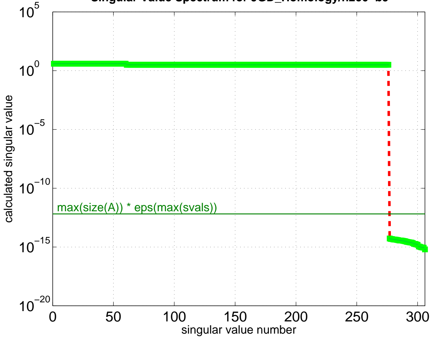
Singular Value Spectrum for JGD_Homology/n2c6-b9
