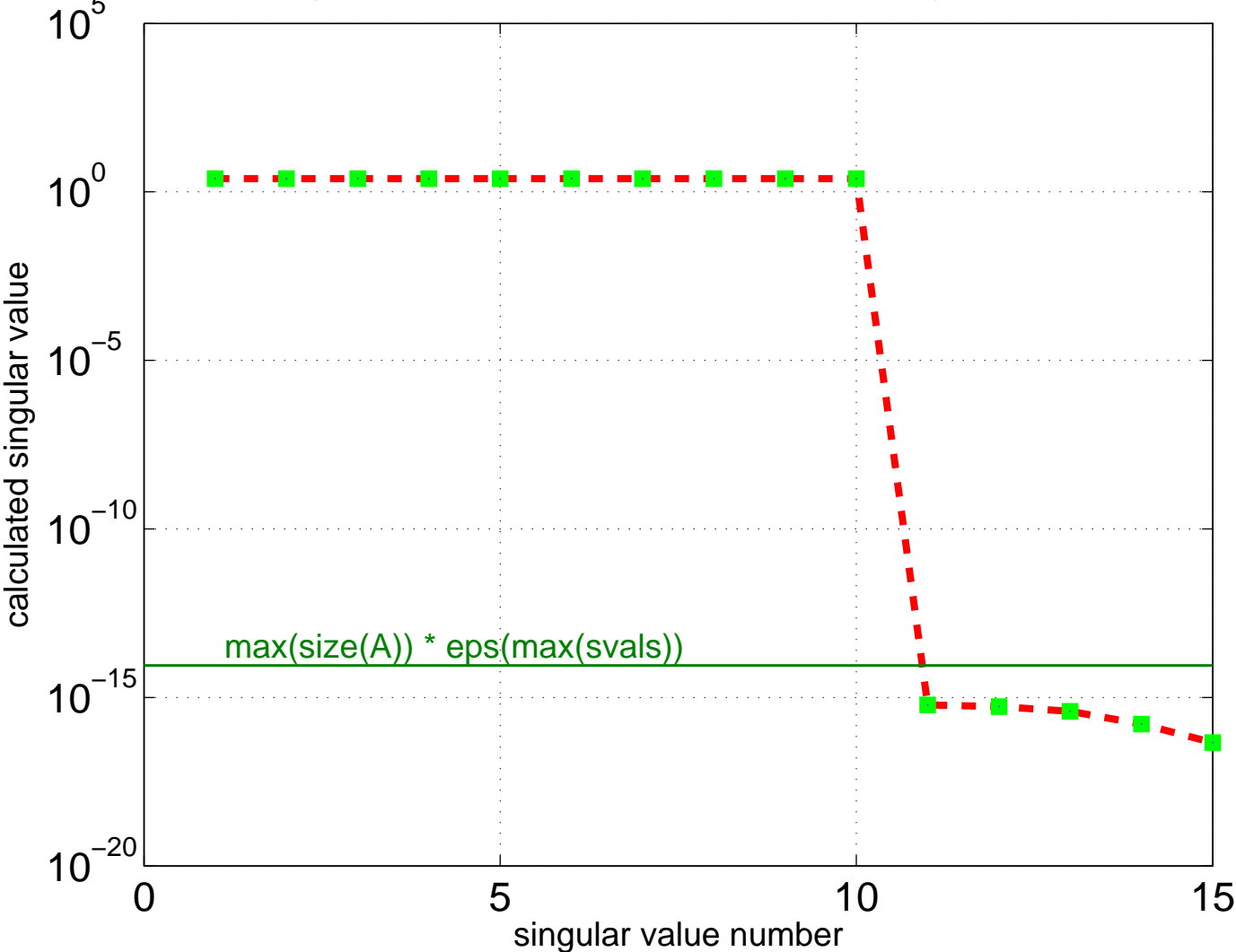
Singular Value Spectrum for JGD_Homology/n3c4-b3
