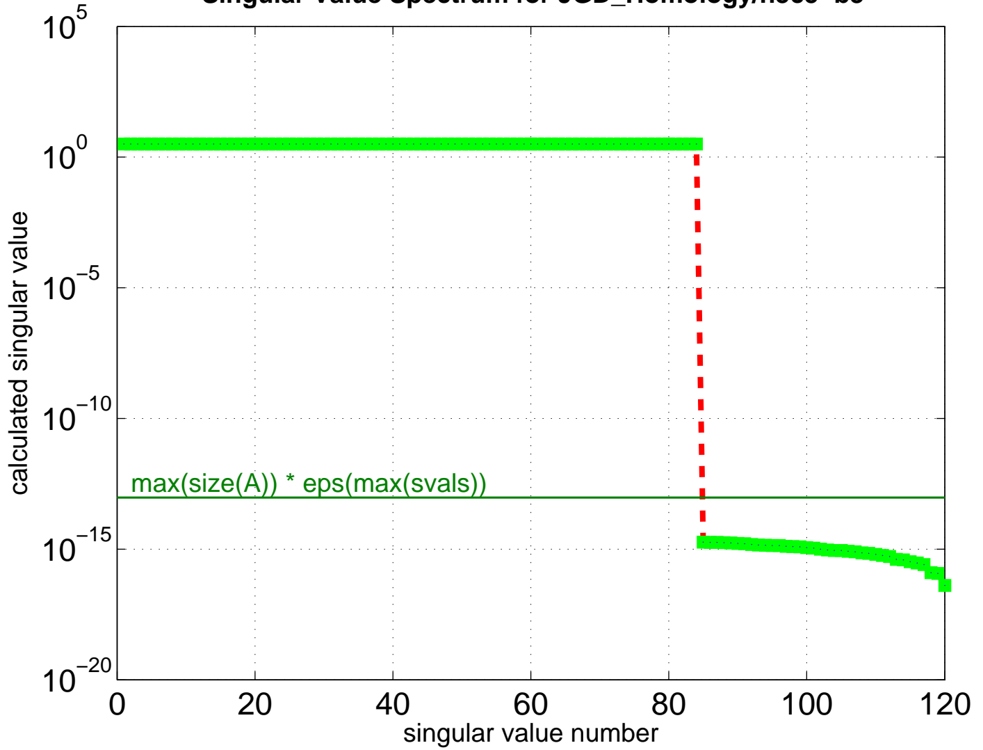
Singular Value Spectrum for JGD_Homology/n3c5-b3
