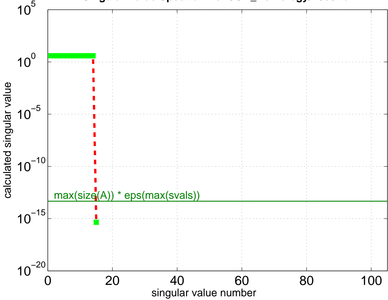
Singular Value Spectrum for JGD_Homology/n3c6-b1
