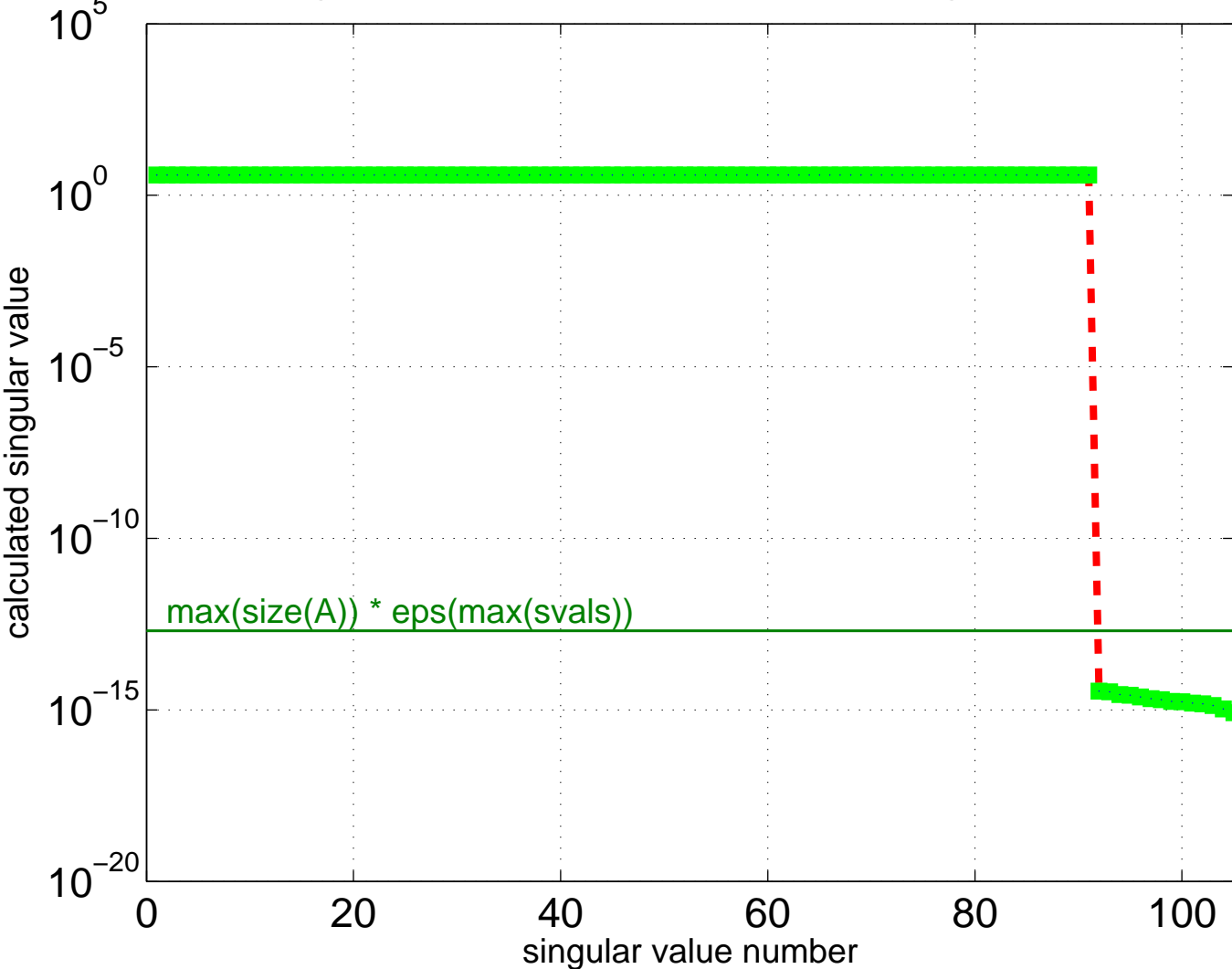
Singular Value Spectrum for JGD_Homology/n4c5-b2
