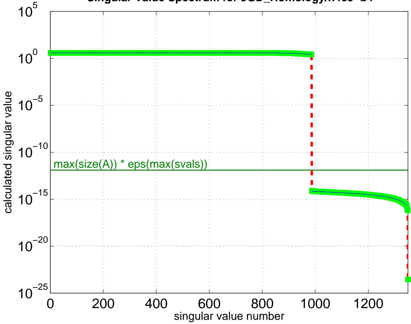
Singular Value Spectrum for JGD_Homology/n4c5-b4
