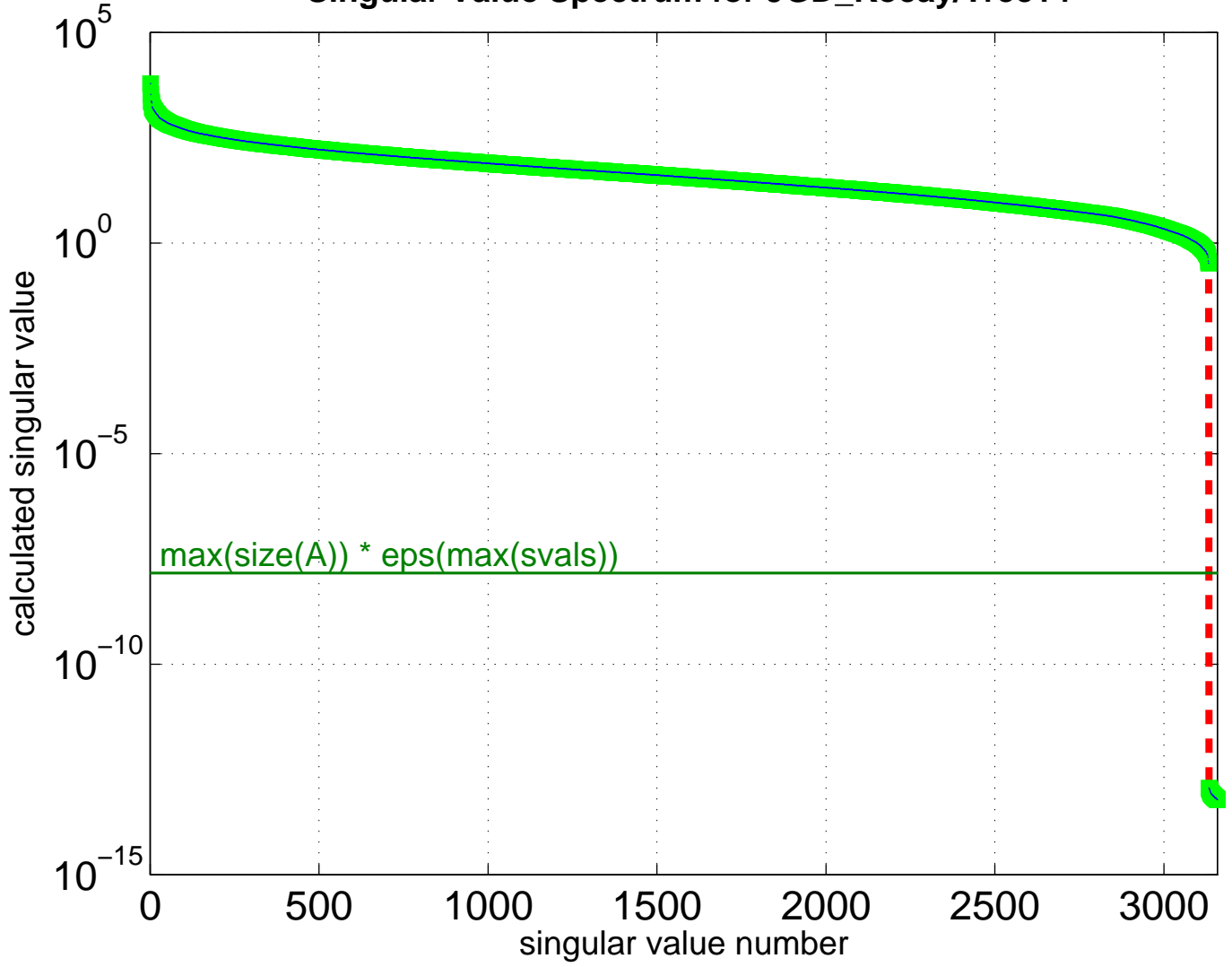
Singular Value Spectrum for JGD_Kocay/Trec14
