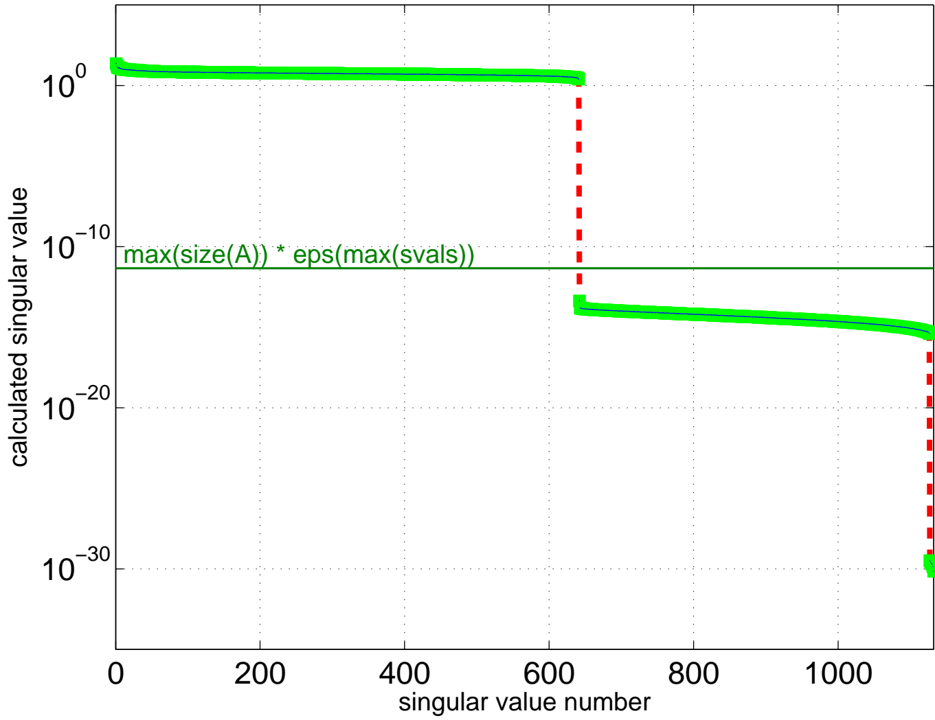
Singular Value Spectrum for JGD_SL6/D_8
