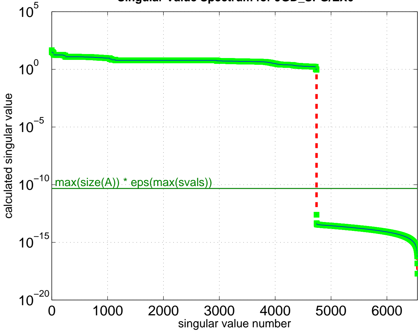
Singular Value Spectrum for JGD_SPG/EX6
