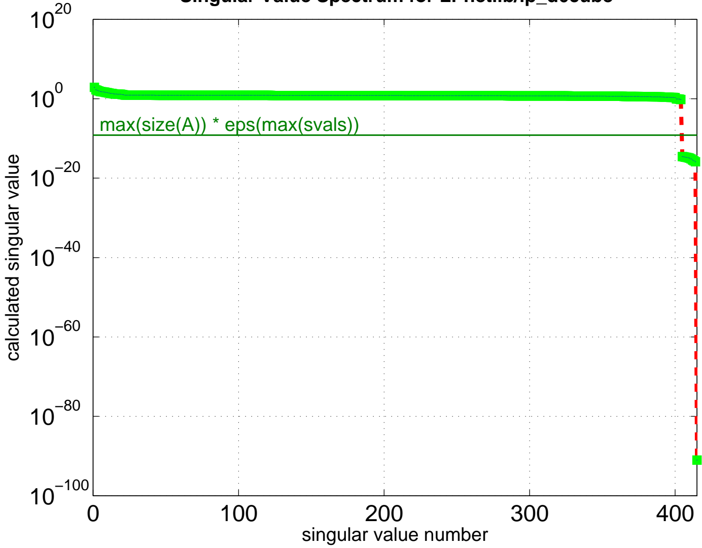
Singular Value Spectrum for LPnetlib/lp_d6cube
