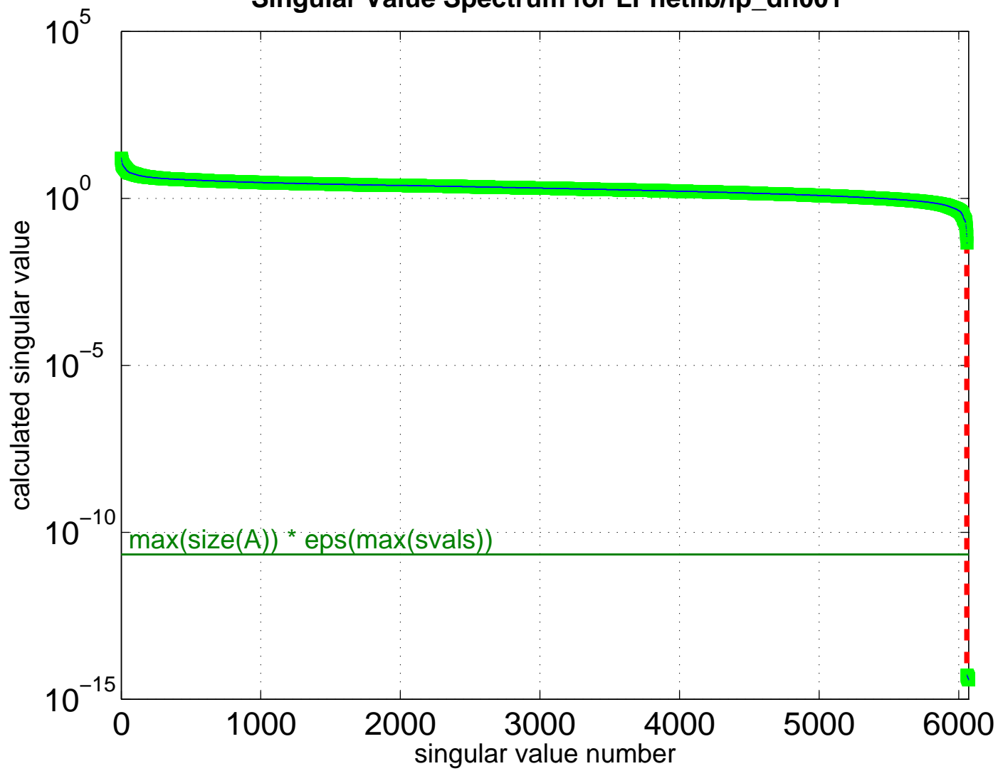
Singular Value Spectrum for LPnetlib/lp_dfl001
