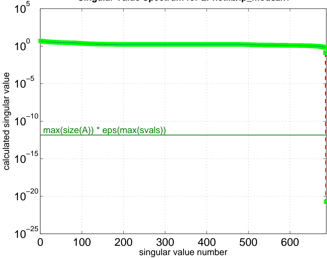
Singular Value Spectrum for LPnetlib/lp_modszk1
