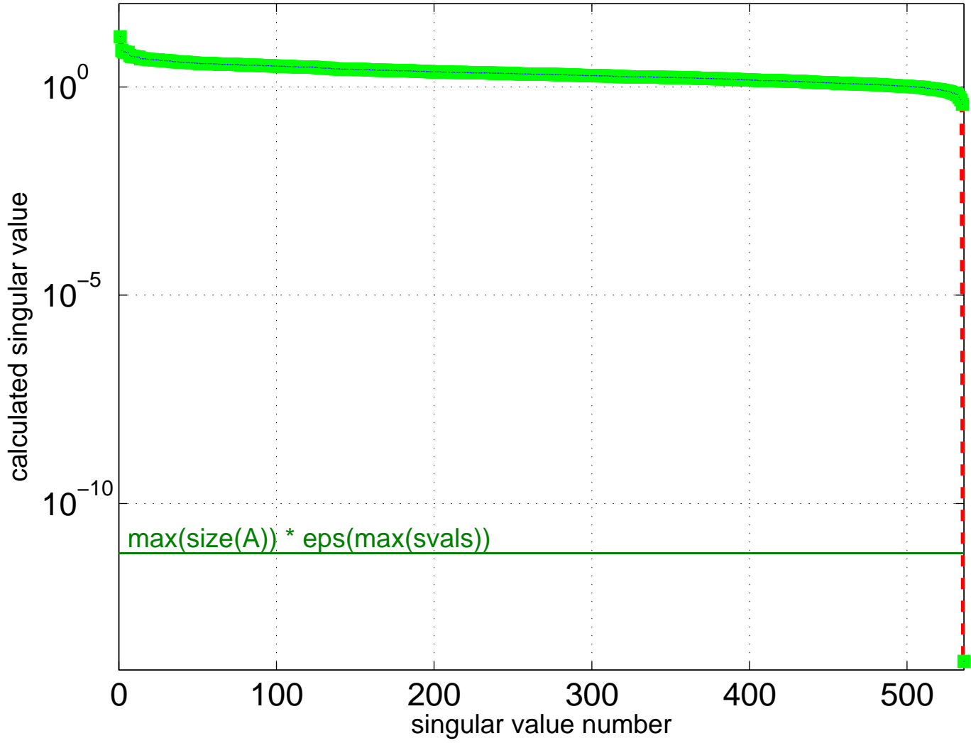
Singular Value Spectrum for LPnetlib/lp_shell
