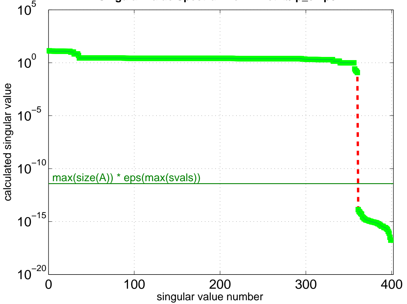
Singular Value Spectrum for LPnetlib/lp_ship04l
