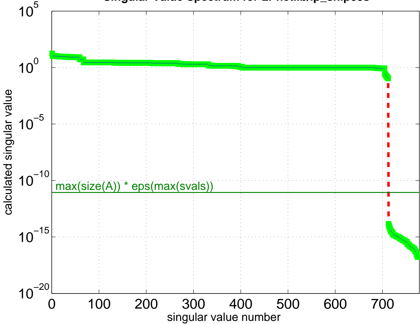
Singular Value Spectrum for LPnetlib/lp_ship08s
