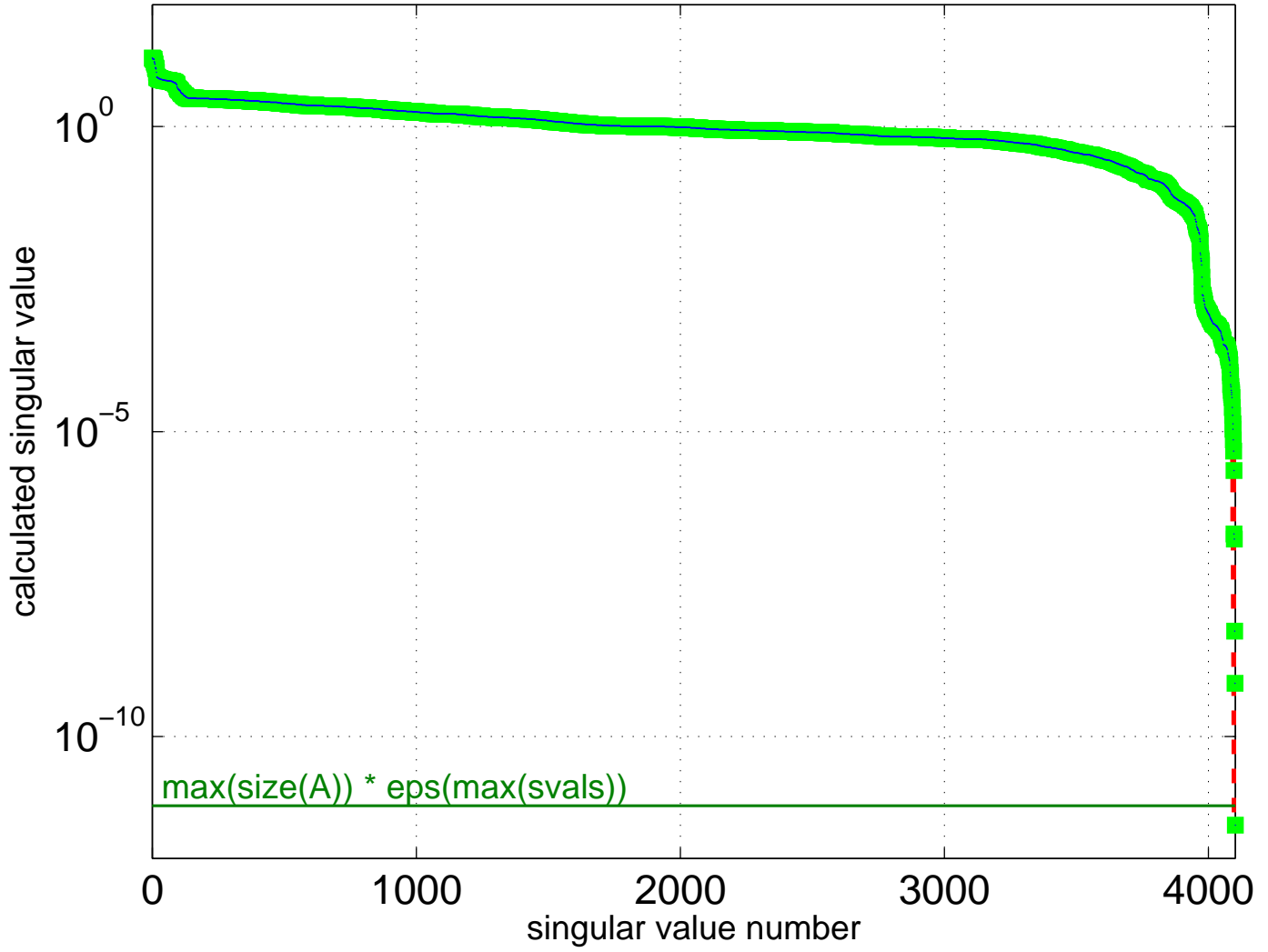
Singular Value Spectrum for Mallya/lhr04c
