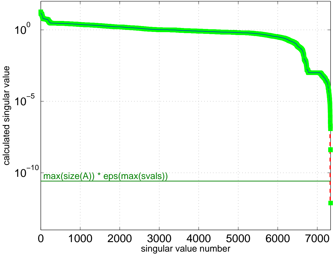
Singular Value Spectrum for Mallya/lhr07c
