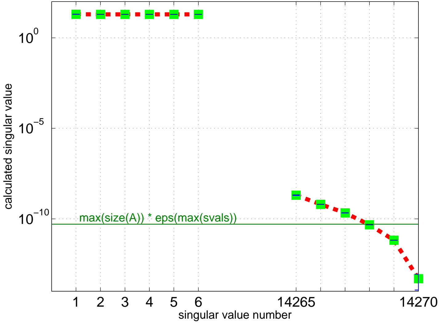
Partial Singular Value Spectrum for Mallya/lhr14c
