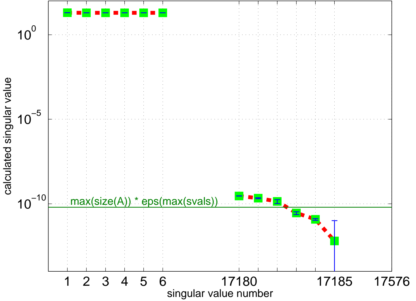
Partial Singular Value Spectrum for Mallya/lhr17
