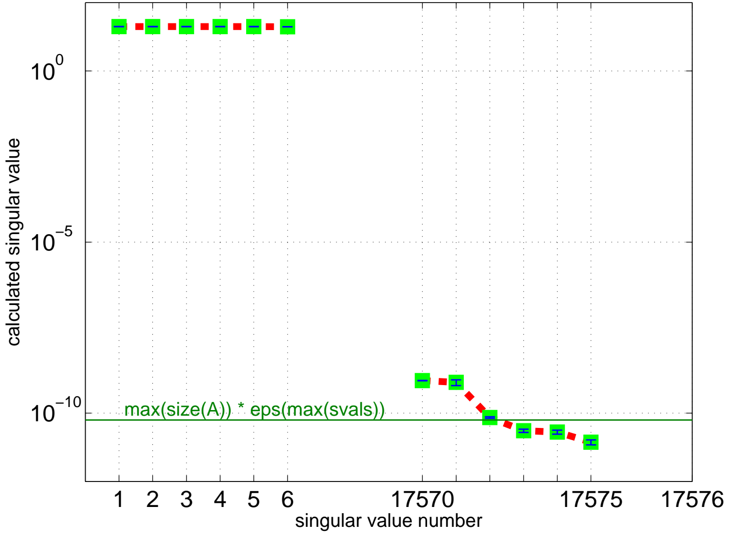
Partial Singular Value Spectrum for Mallya/lhr17c
