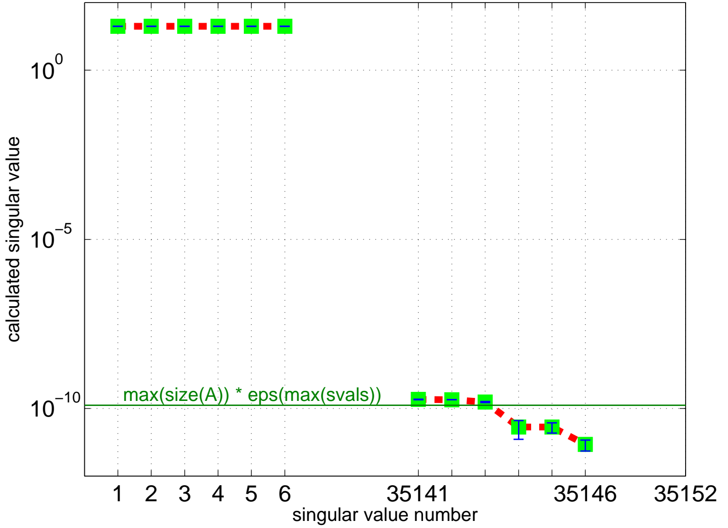
Partial Singular Value Spectrum for Mallya/lhr34c
