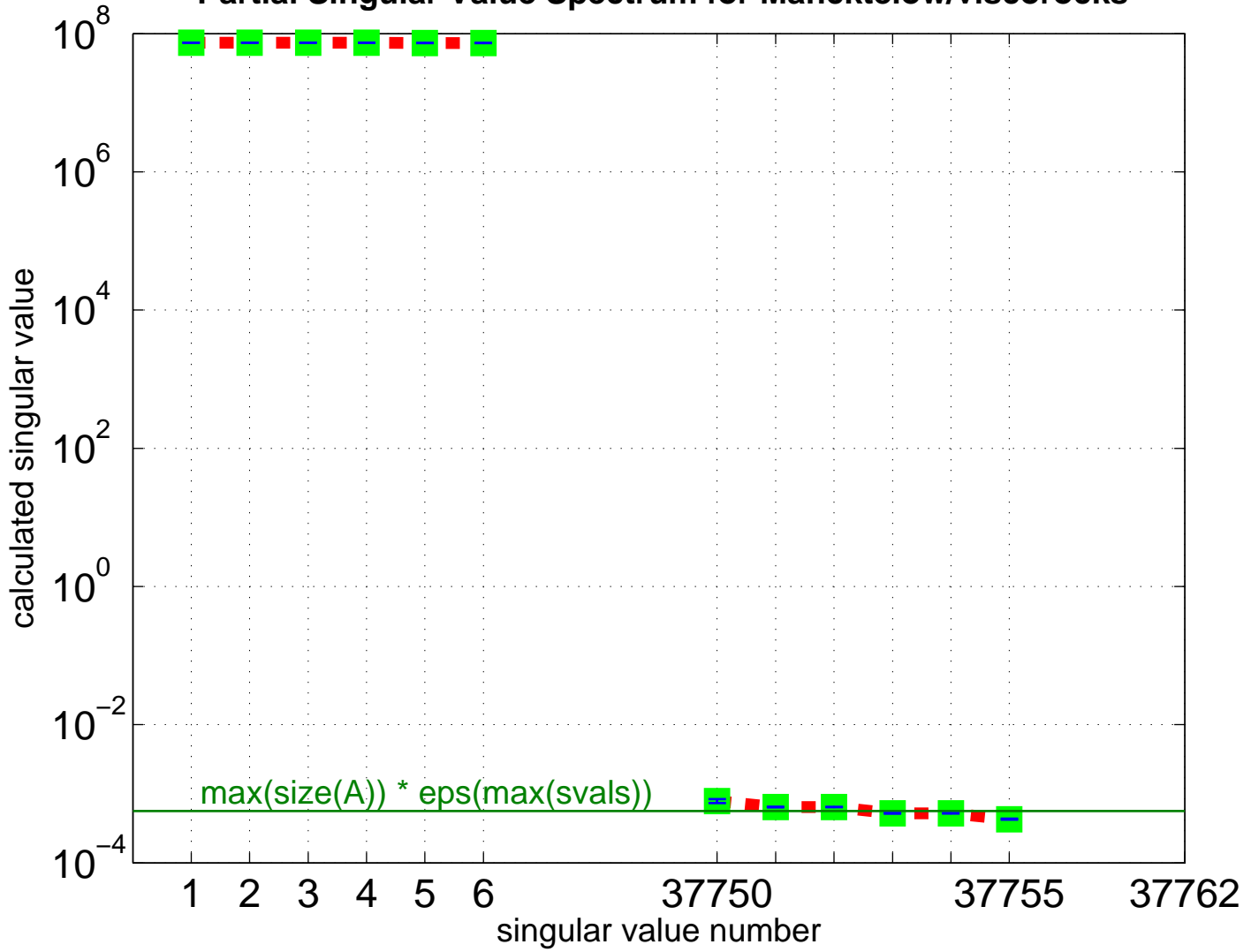
Partial Singular Value Spectrum for Mancktelow/viscorocks
