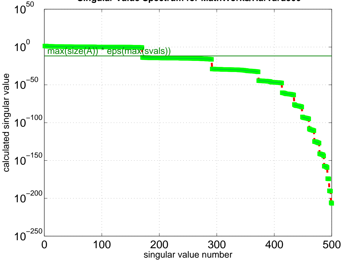
Singular Value Spectrum for MathWorks/Harvard500
