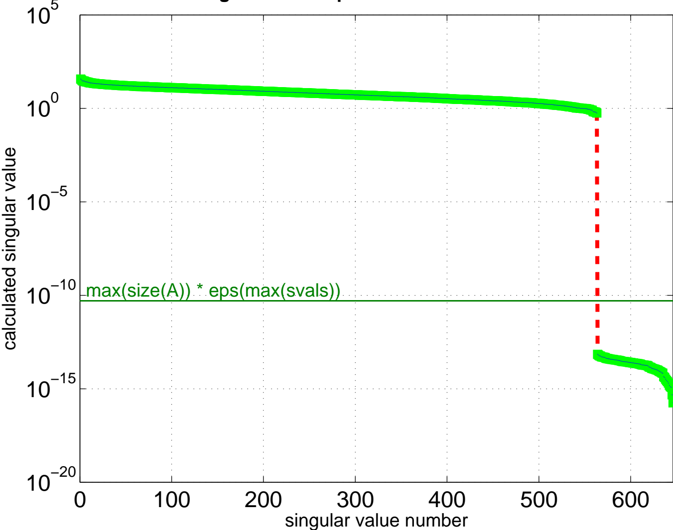
Singular Value Spectrum for Meszaros/aa6
