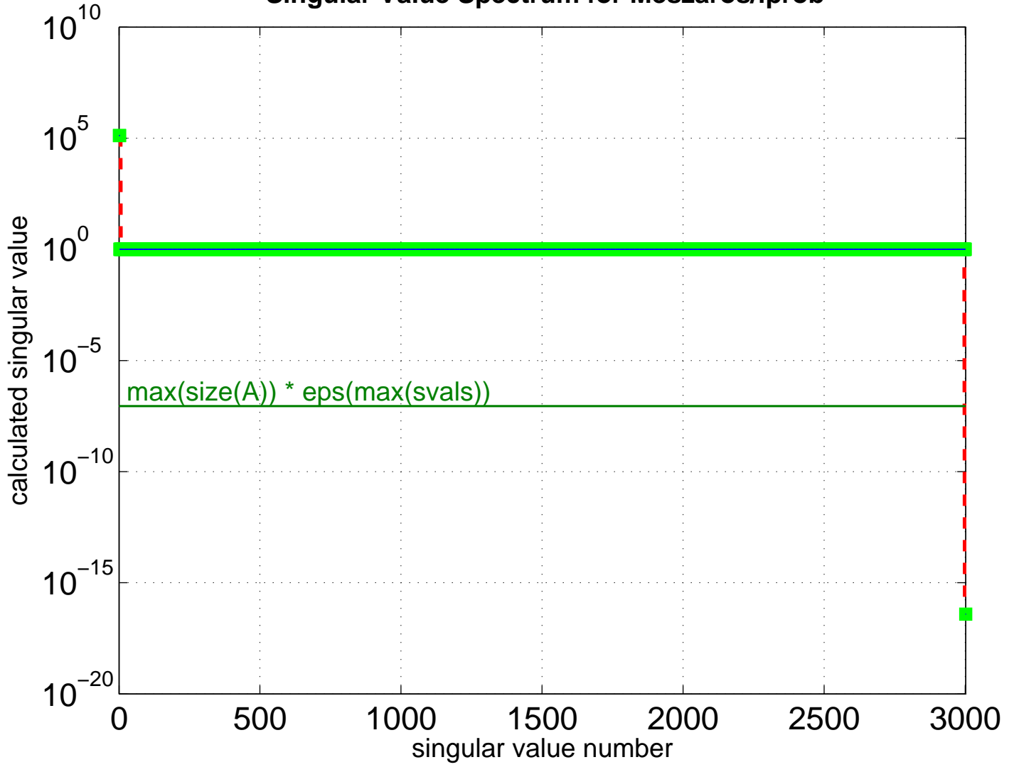
Singular Value Spectrum for Meszaros/ipro
