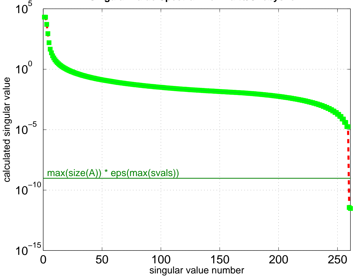
Singular Value Spectrum for Muite/Chebyshev1
