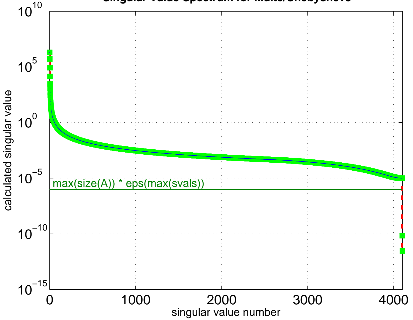
Singular Value Spectrum for Muite/Chebyshev3
