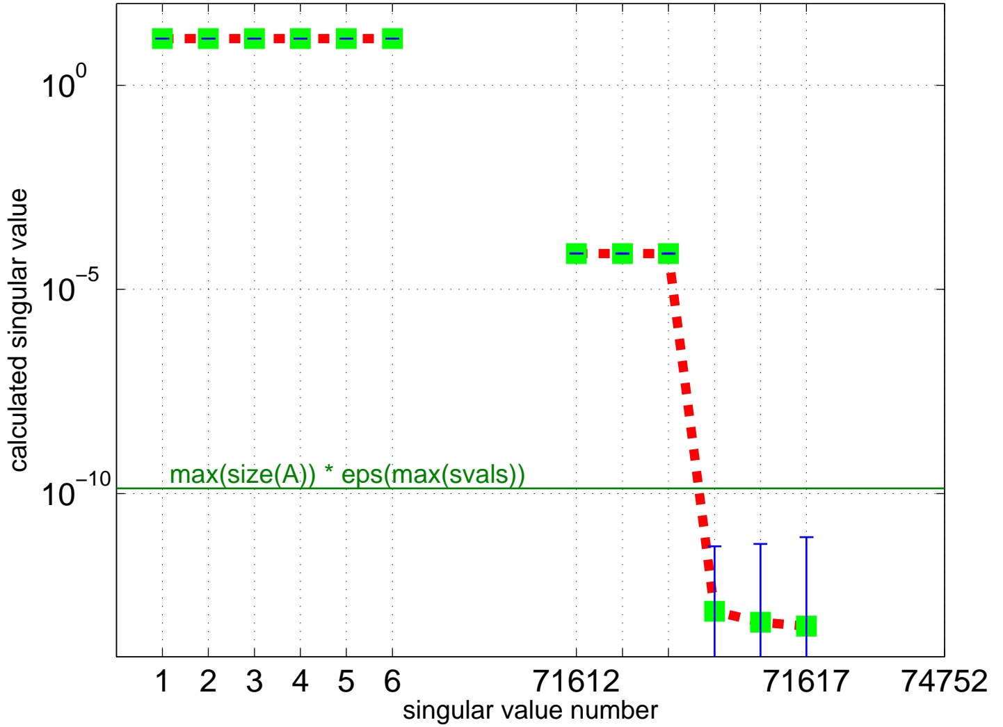
Partial Singular Value Spectrum for Mulvey/pfinan512
