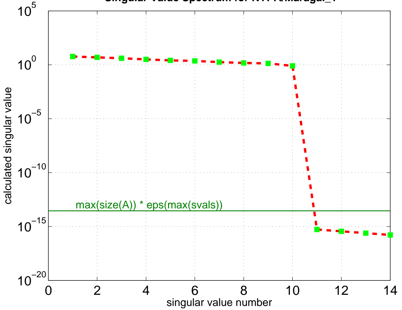
Singular Value Spectrum for NYPA/Maragal_1
