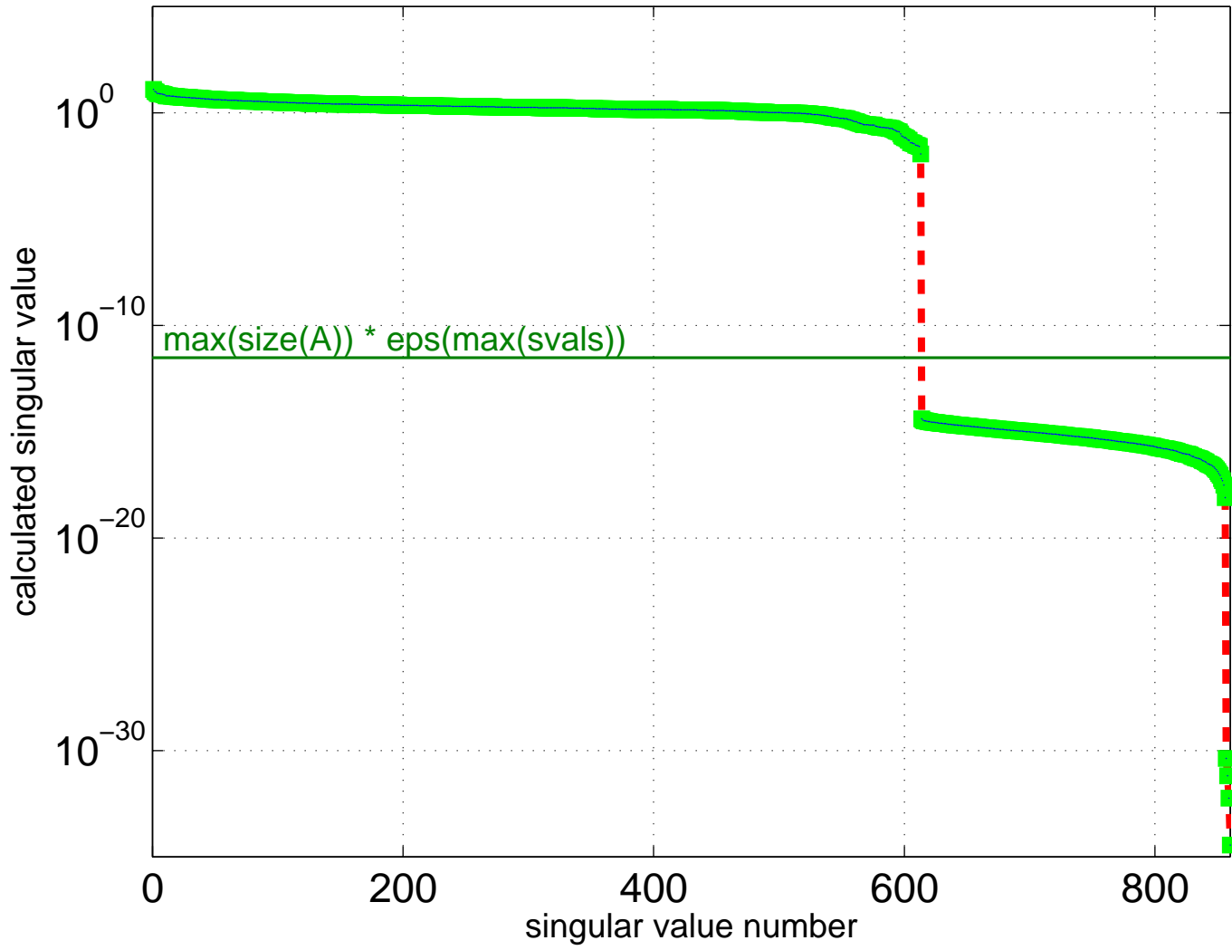
Singular Value Spectrum for NYPA/Maragal_3
