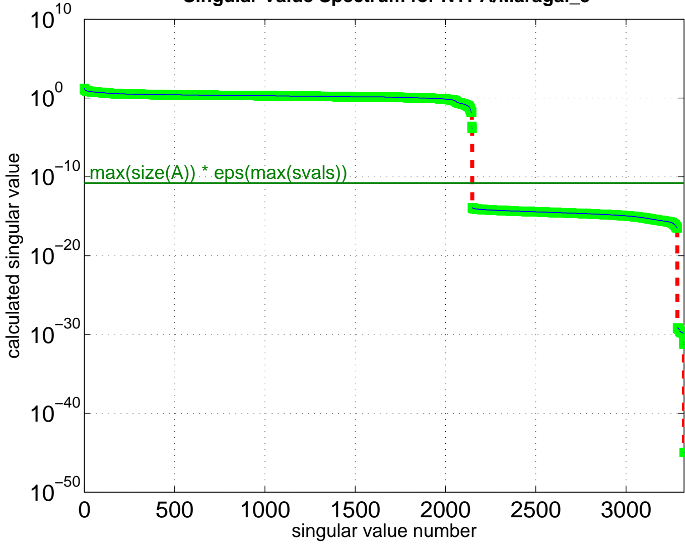
Singular Value Spectrum for NYPA/Maragal_5
