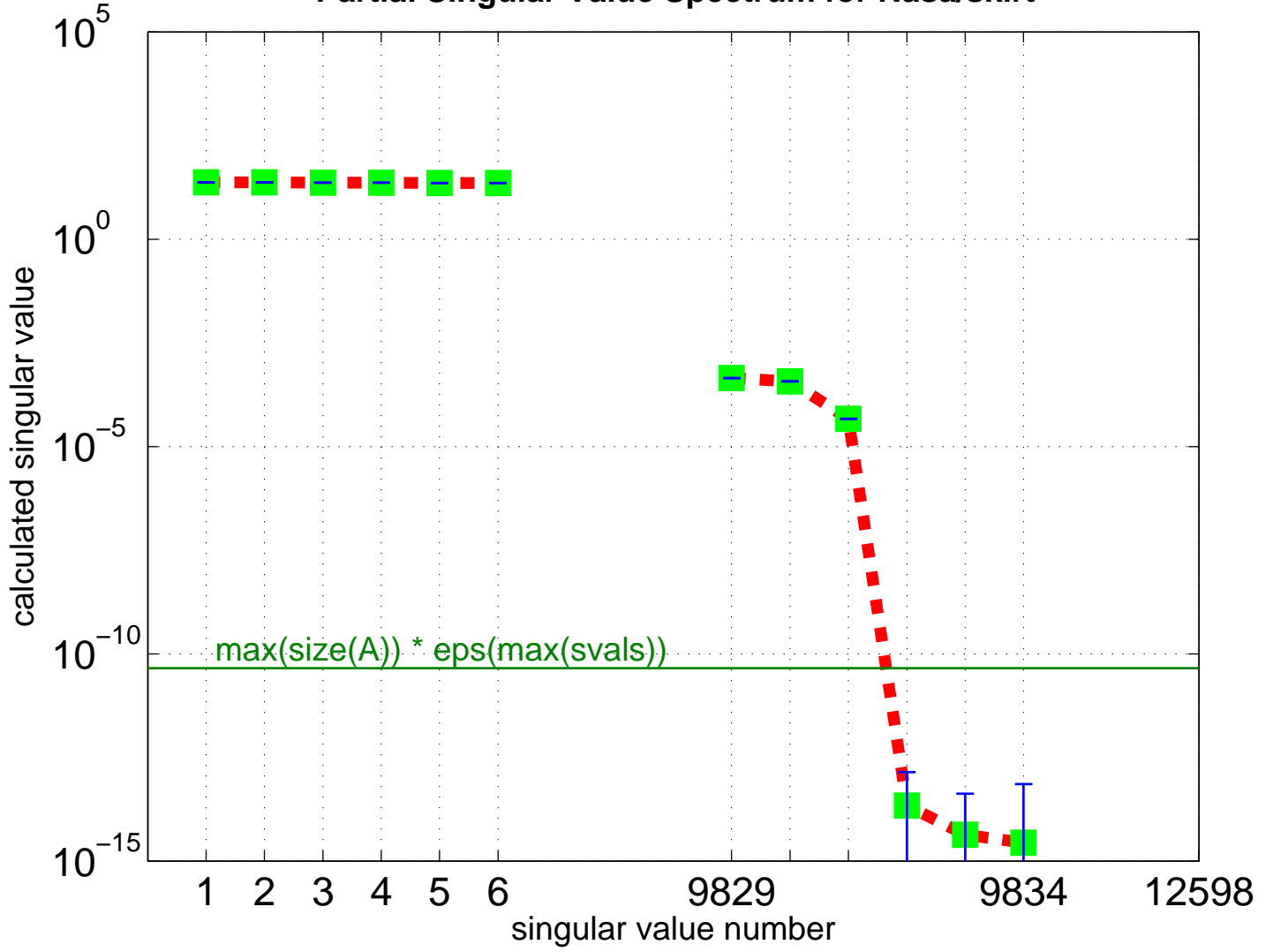
Partial Singular Value Spectrum for Nasa/skirt
