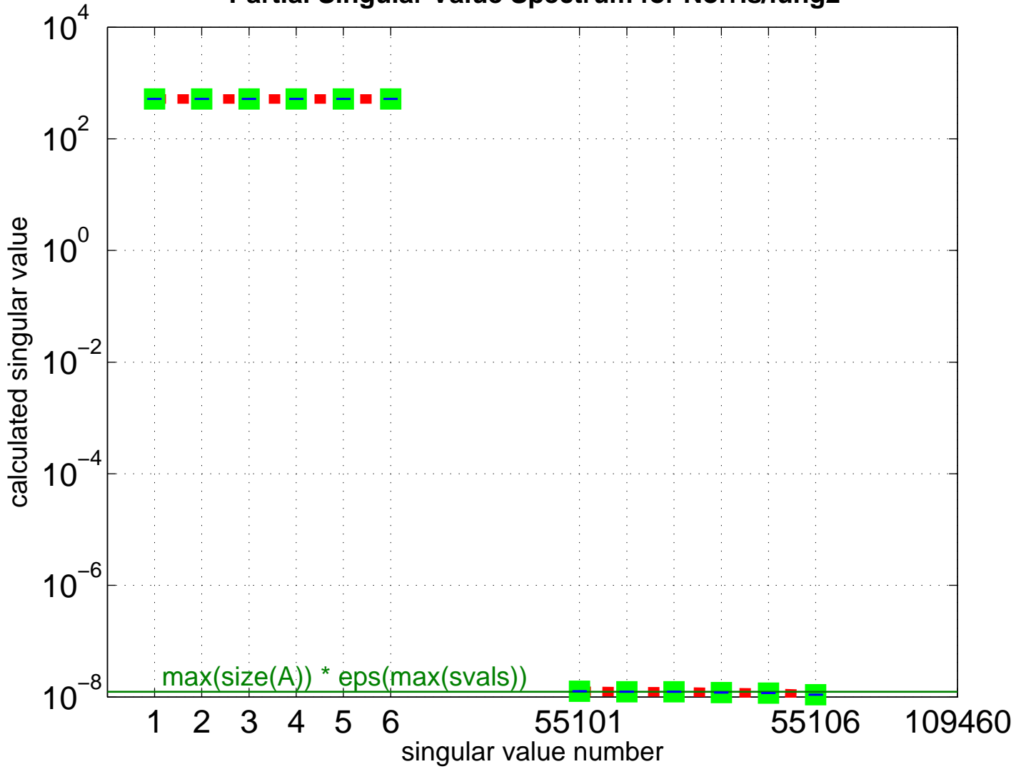
Partial Singular Value Spectrum for Norris/lung2
