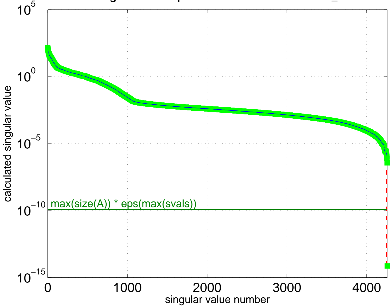
Singular Value Spectrum for Oberwolfach/t2dal_a
