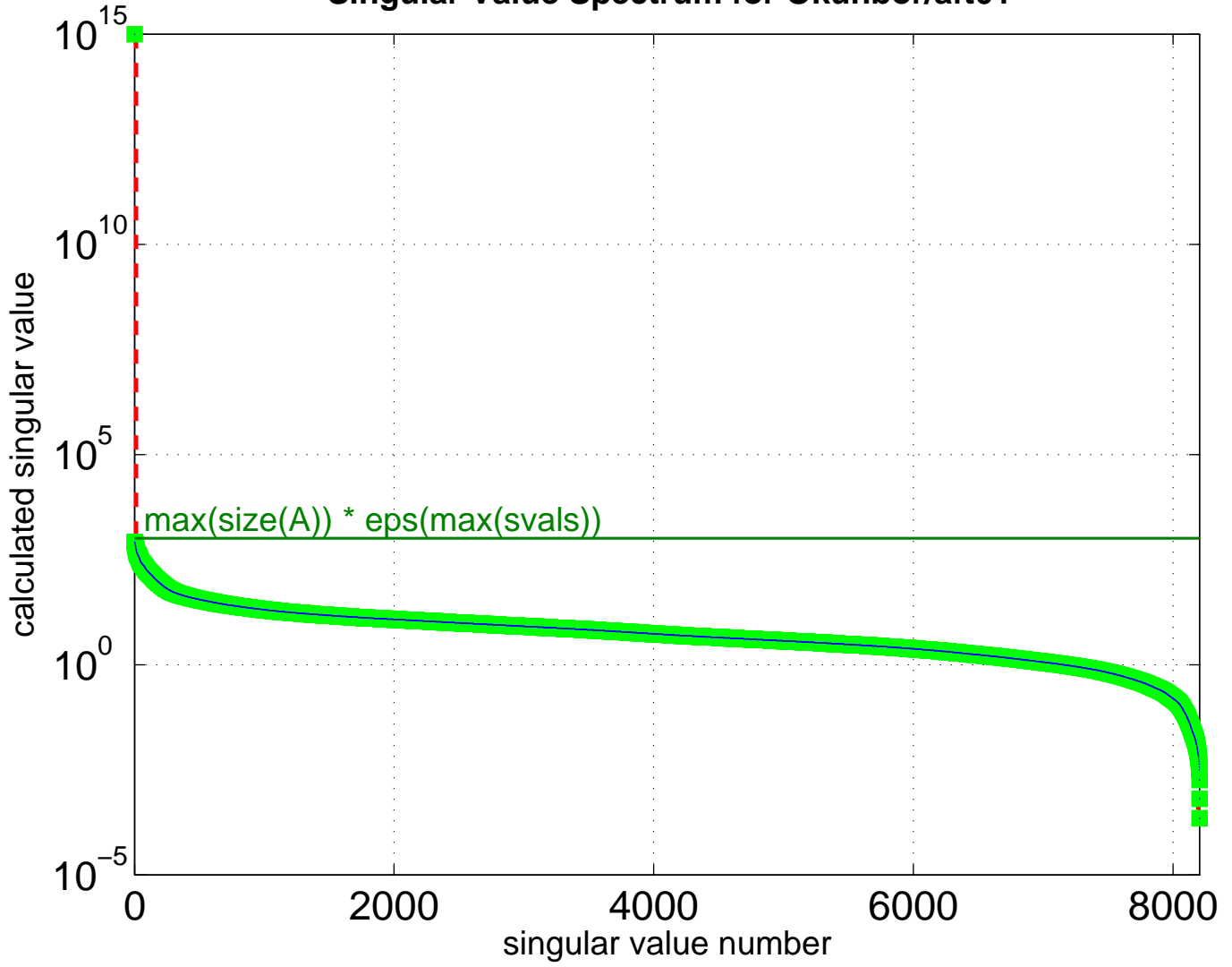
Singular Value Spectrum for Okunbor/aft01
