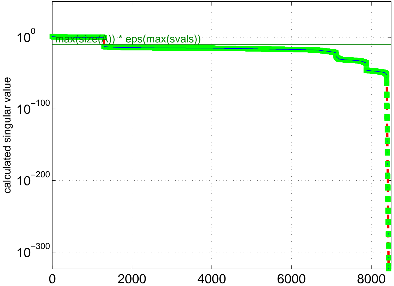
Singular Value Spectrum for Pajek/EVA
